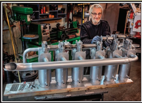
Kerwin Davison shown in his workshop working on the full size replica of the Handley Page V-12 engine which he completed in 2019. The engine was in a plane which crash landed in Parrsboro in 1919.
